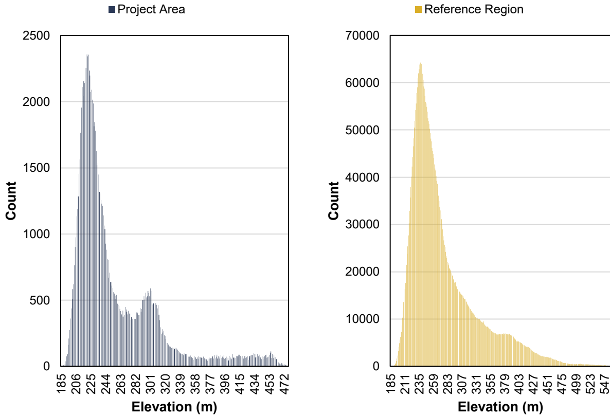
Figure 3.9: Elevation distribution in the Project Area (blue graph, on the left) and Reference Region (orange graph, on the right)
