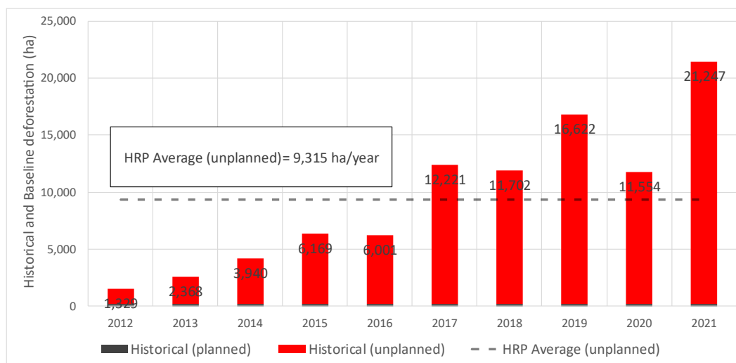
Figure 3.28. Annual deforestation in the reference region during the historical period.
