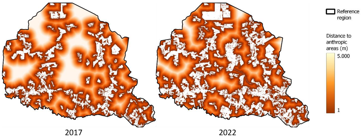
Figure 3.34. Factor maps: distance to anthropic areas (connected patches larger than 100 ha).
