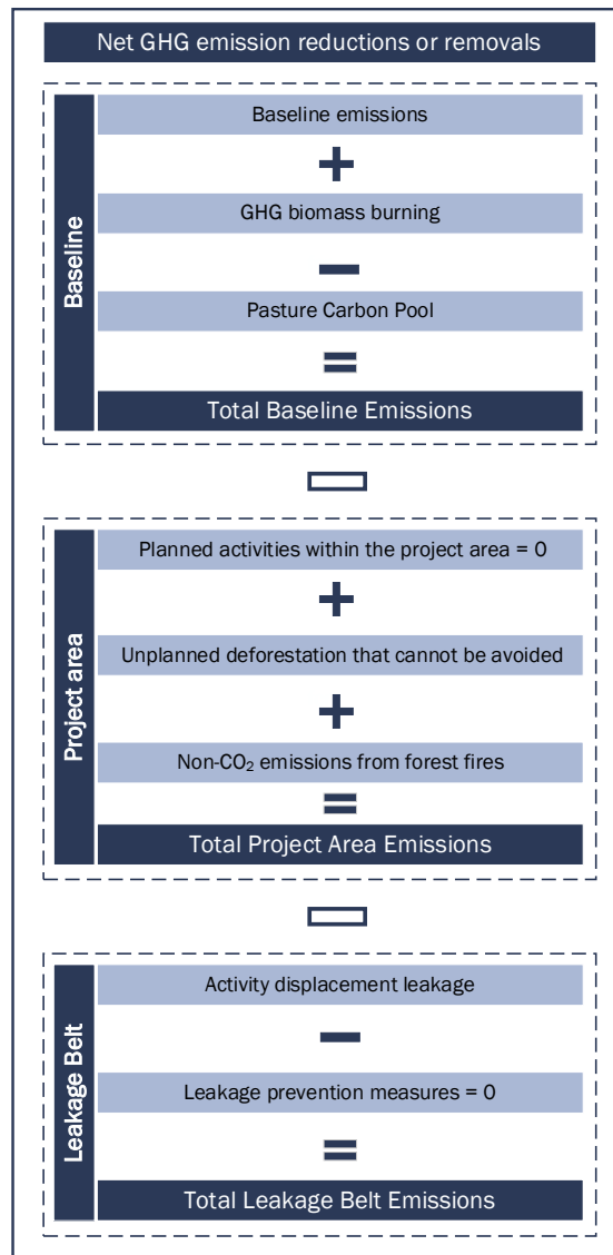
Figure 4.5. Summary of the calculation of Net GHG emission reductions or removals
