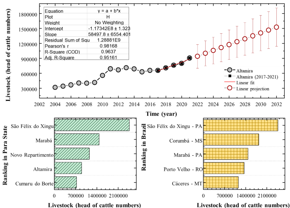
Figure 3.24. Top: herd size in the Altamira municipality as a function of time and linear extrapolation to future years. Bottom: ranking of livestock production in the state of Pará (left) and Brazil (right) by municipality, according to 2021 data (the state abbreviations are: Pará (PA), Mato Grosso do Sul (MS), Rondônia (RO), and Mato Grosso (MT)). Source: IBGE (2021b).
