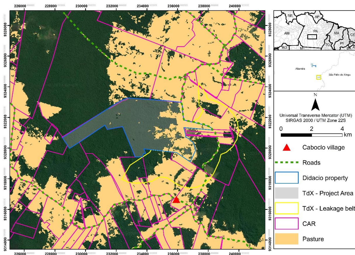
Figure 1.15. Access roads to the leakage belt and surrounding areas.
