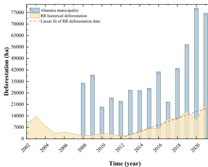
Figure 3.23. A comparison between the annual deforestation curves in the Altamira municipality, where the project is located, and in the reference region.
