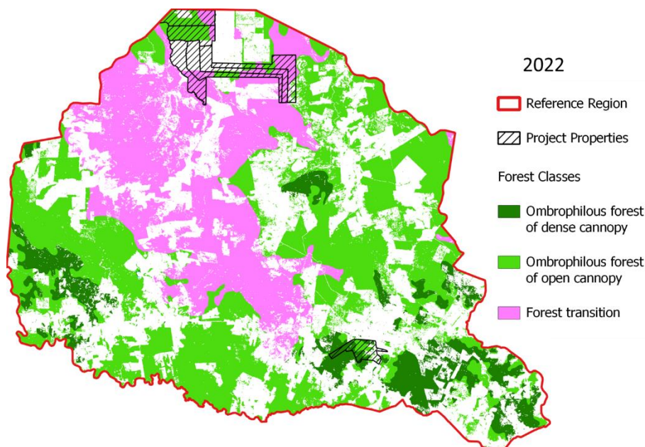
Figure 3.18. Forest classes at forested areas within the RR at the project start date.
