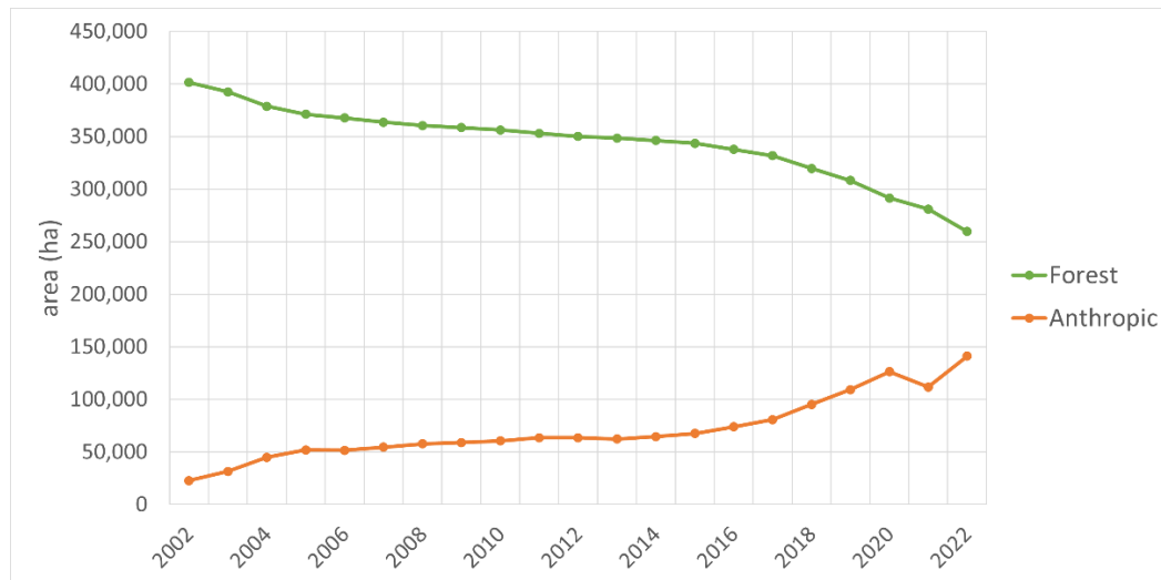
Figure 3.25. The evolution of Forest and Anthropic classes in the project's reference region during the extended historical period (the Anthropic class consists essentially of pasturelands).
