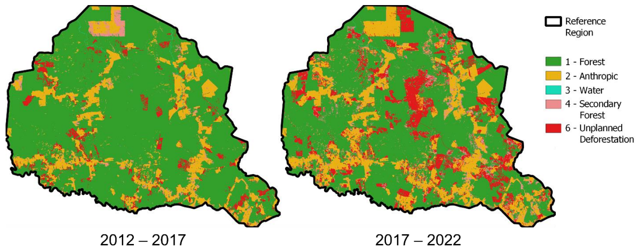
Figure 3.20. Half-historical-period deforestation maps.
