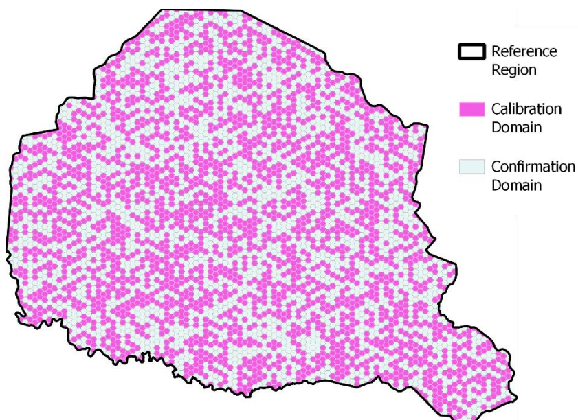
Figure 3.40. Spatial domains used for model calibration and confirmation.
