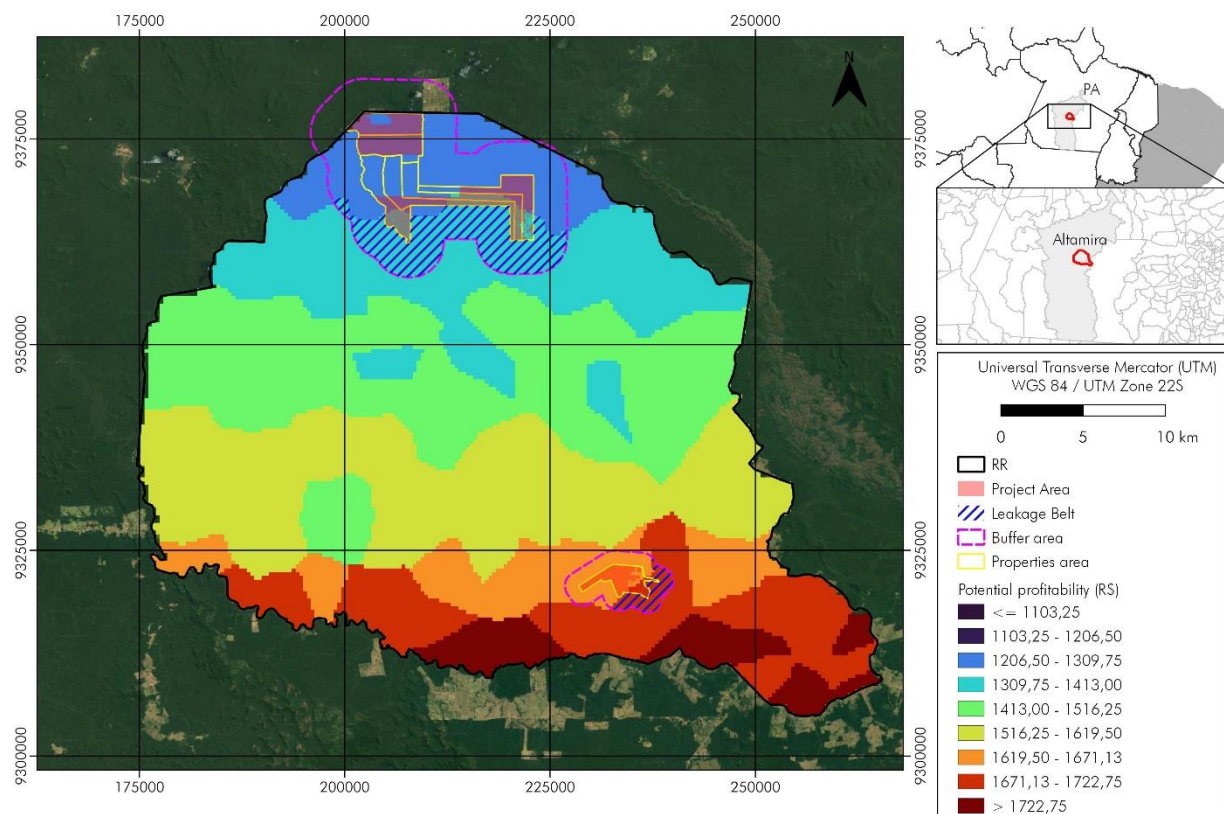
Figure 3.14: Potential profitability in Reference Region, and delimited leakage belt where there are highest values to potential profitability, and their respective buffers.
