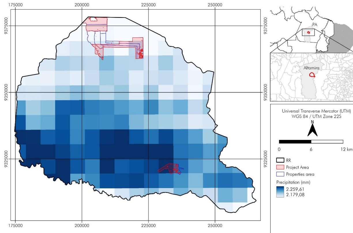
Figure 3.7: Average annual precipitation in the Reference Region and Project Area.
