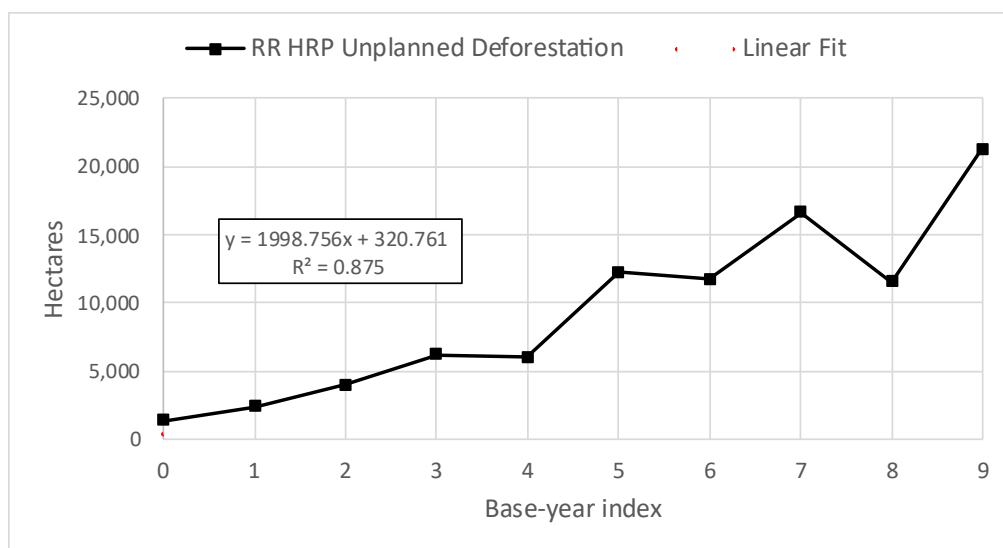
Figure 3.29. Historical unplanned deforestation in the reference region and linear fit.
