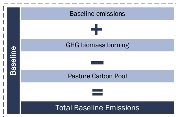
Figure 4.2. Schematic of total baseline emissions estimation
