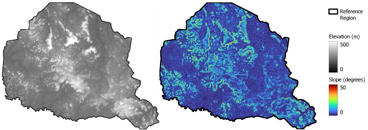
Figure 3.33. Factor maps: elevation and slope.
