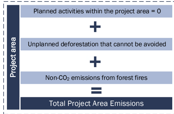
Figure 4.3. The total project area emissions estimation
