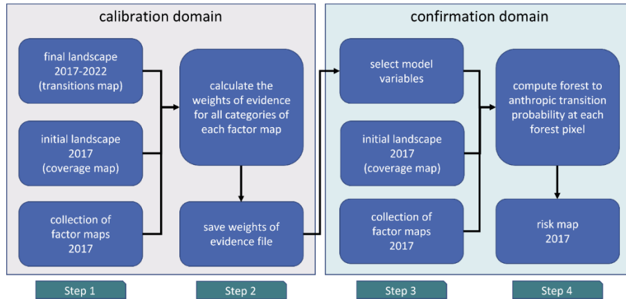
Figure 3.38. Flow chart explaining the construction of risk maps for model accuracy assessment using the “spatial domains” approach for model calibration and confirmation.
