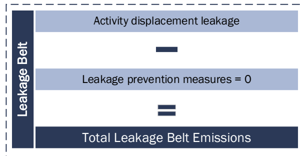
Figure 4.4. Leakage belt ex-ante estimation
