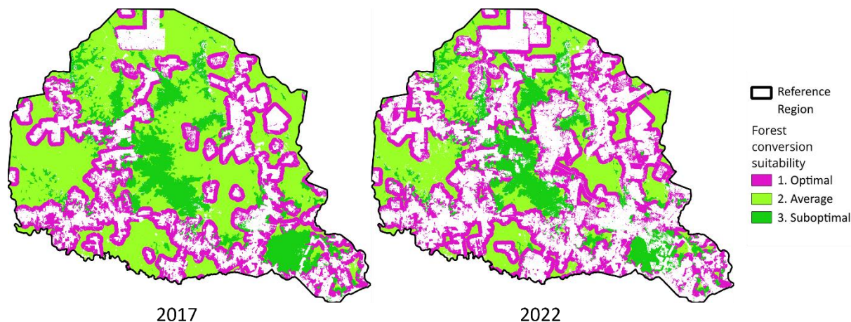
Figure 3.37. Factor maps: suitability zones.
