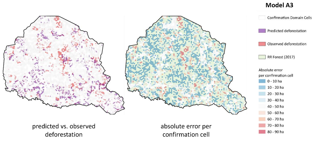
Figure 3.41. Accuracy assessment of Model A3.
