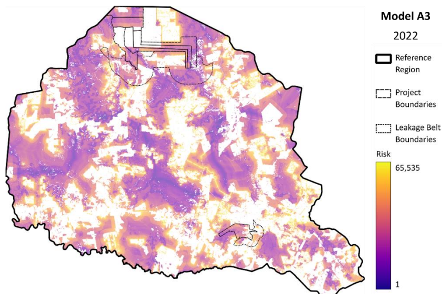
Figure 3.42. Baseline risk map for Model A3.
