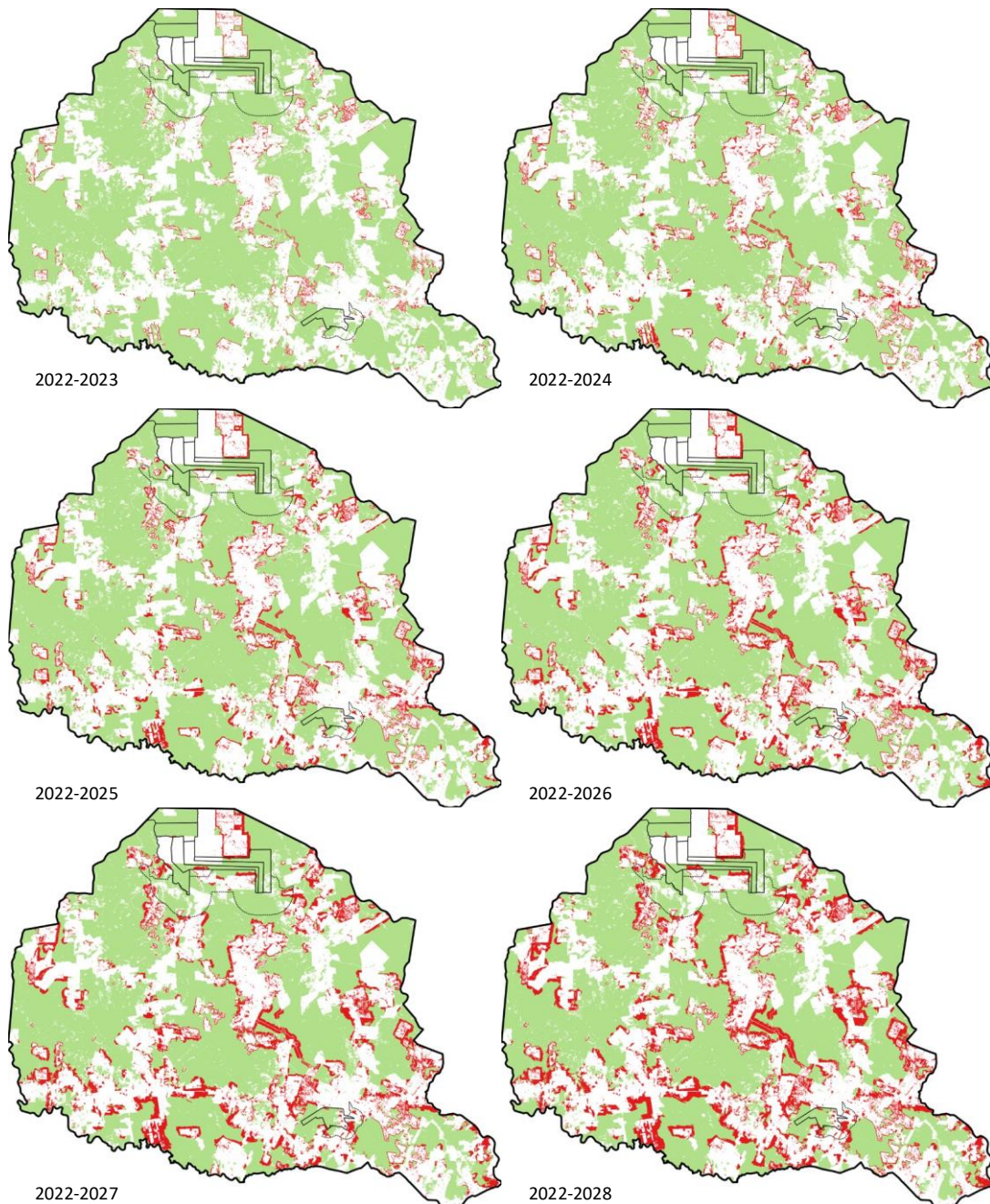
Figure 3.45. Predicted baseline deforestation in the reference region (6 years). Legend code: ■ Baseline deforestation (predicted), ■ Forest.
