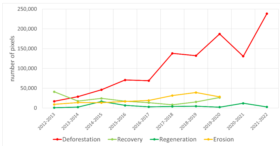
Figure 3.19. Transitions occurring in the reference region during the historical period.
