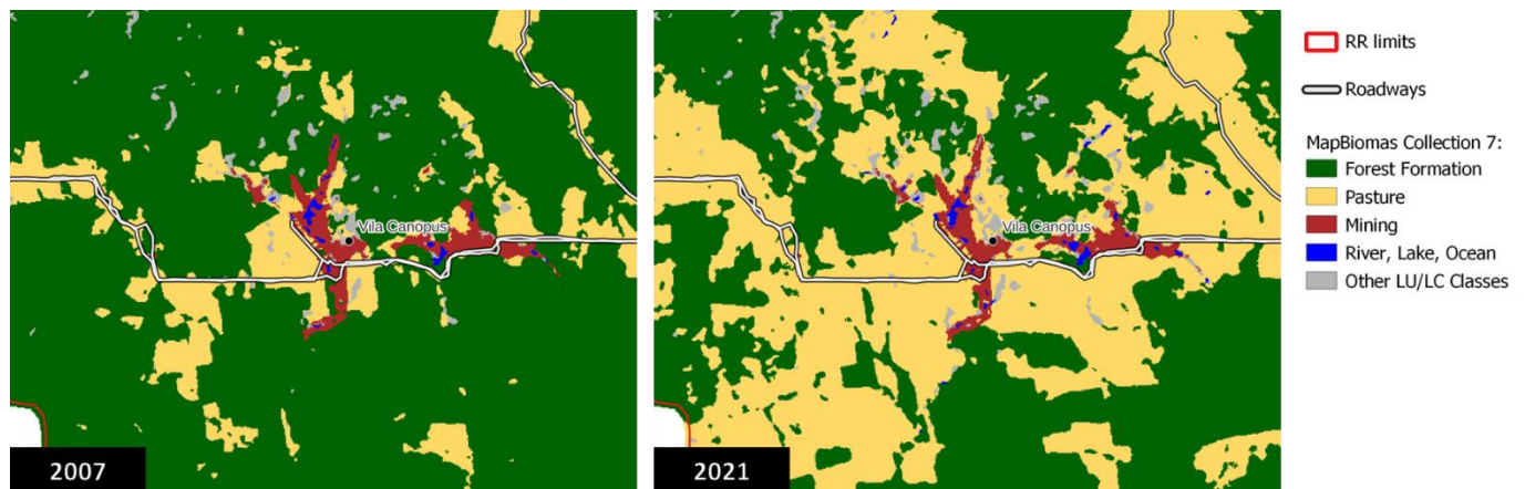
Figure 3.5. Expansion of pastures around the mining site located at Vila Canopus.
