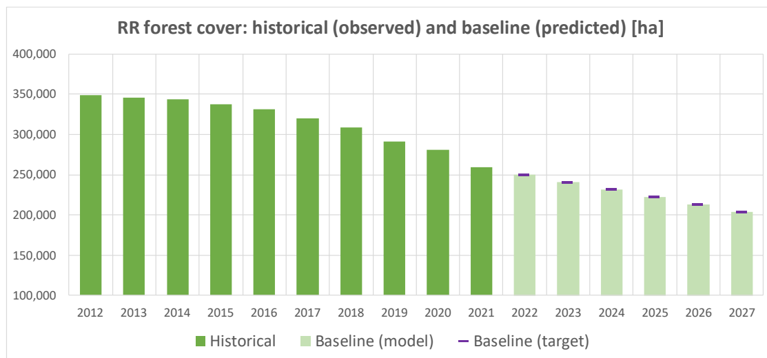
Figure 3.30. Historical evolution of the RR's forest cover (dark-green bars) and the predicted baseline curve – both target baseline values (purple dashes) and final baseline model allocation values (light-green bars) are shown.
