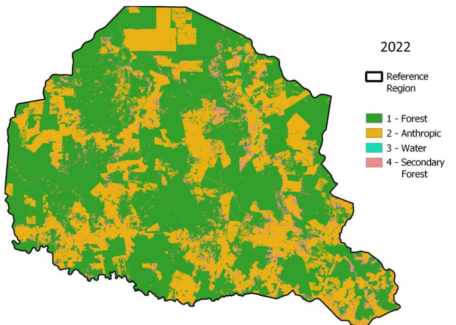
Figure 3.17. Distribution of LU/LC classes in the RR at the project start date.
